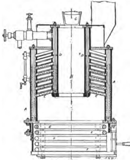
FIG. 160.—Familiar Form of the De Dion Boiler. A is the outer annular chamber connected to the inner annular chamber, B, by the inclined tubes, CC. A screen, DD, separates the steam and water spaces. EE are tubes for pre-heating the feed-water; FF, for superheating the exhaust steam. Steam connections same as in Fig. 157.
